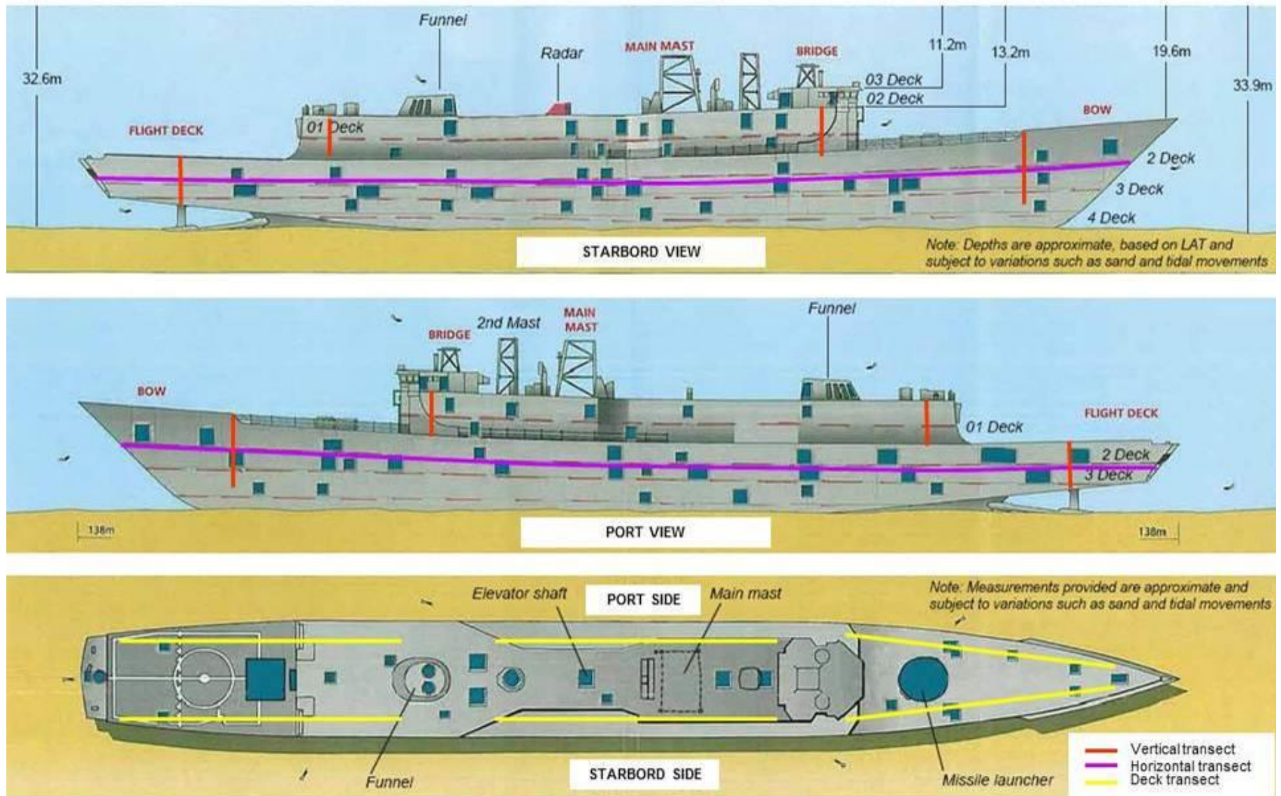
Figure 2: Plans of the Ex-HMAS Adelaide and positions of the reef assemblage survey sampling Transects.
